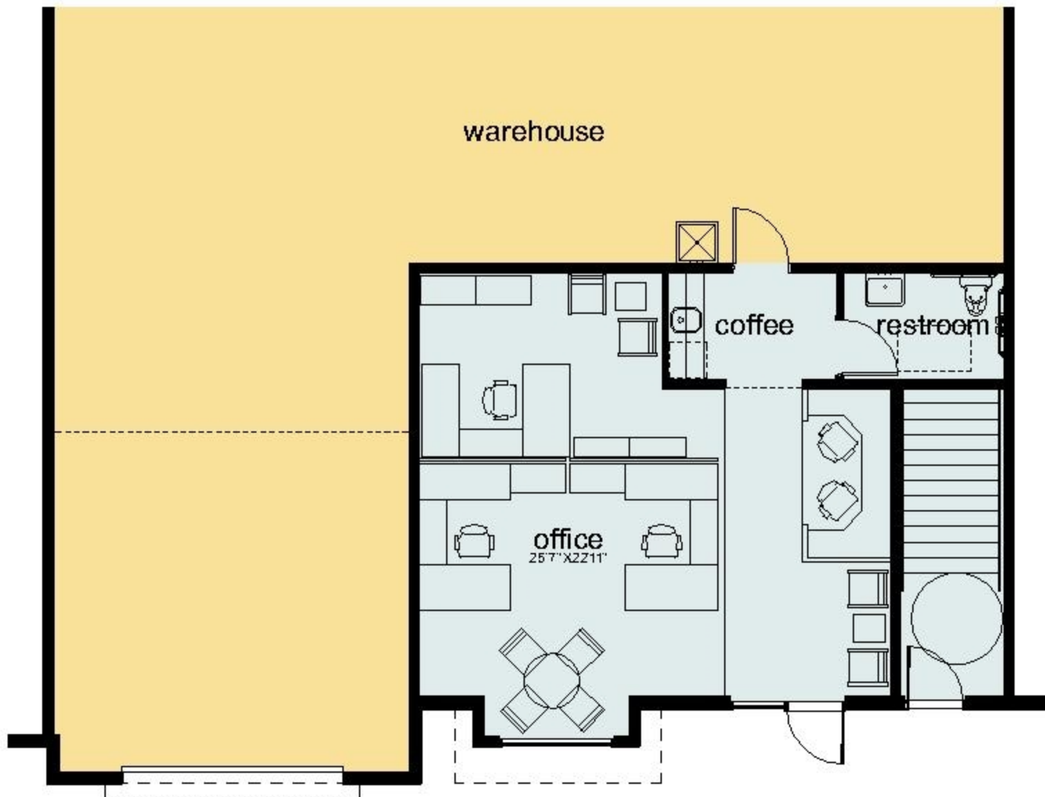
1st Floor Plan - Building 'C1'
